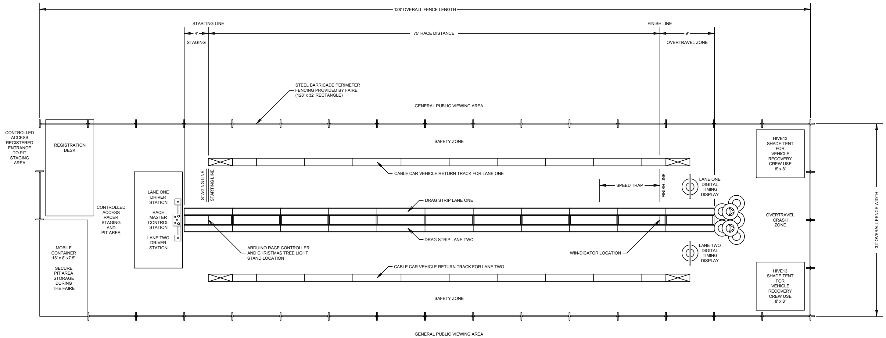
HIVE13 AND FRIENDS POWER TOOL DRAG RACING GENERAL LAYOUT, 2016-02-13
